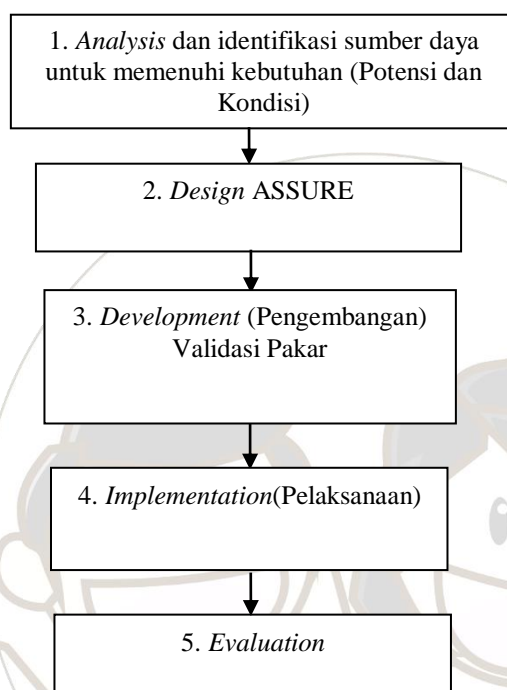
Gambar 1 Prosedur Penelitian
