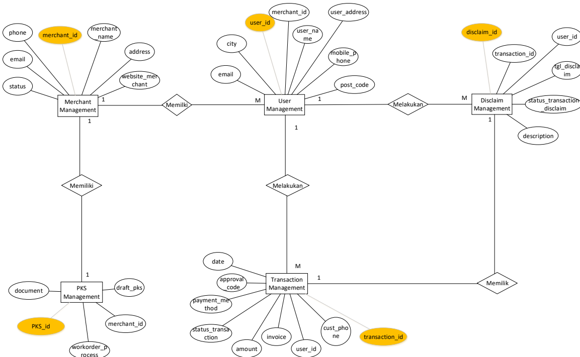
Gambar 3. Entity Relational Diagram
