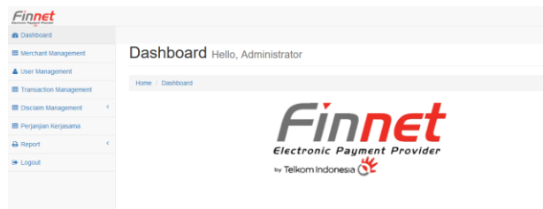
Gambar 7. Dashboard Administrator
