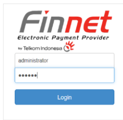
Gambar 6. Form Login
